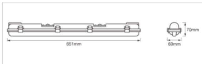
SUBMARINE LED 1X8W 840 60
