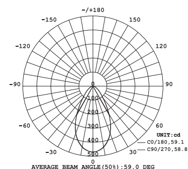
3000K LUMINOUS INTENSITY DISTRIBUTION DIAGRAM
